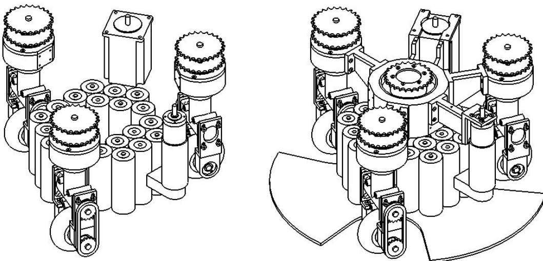
Fig.4.20 Supporting frame
