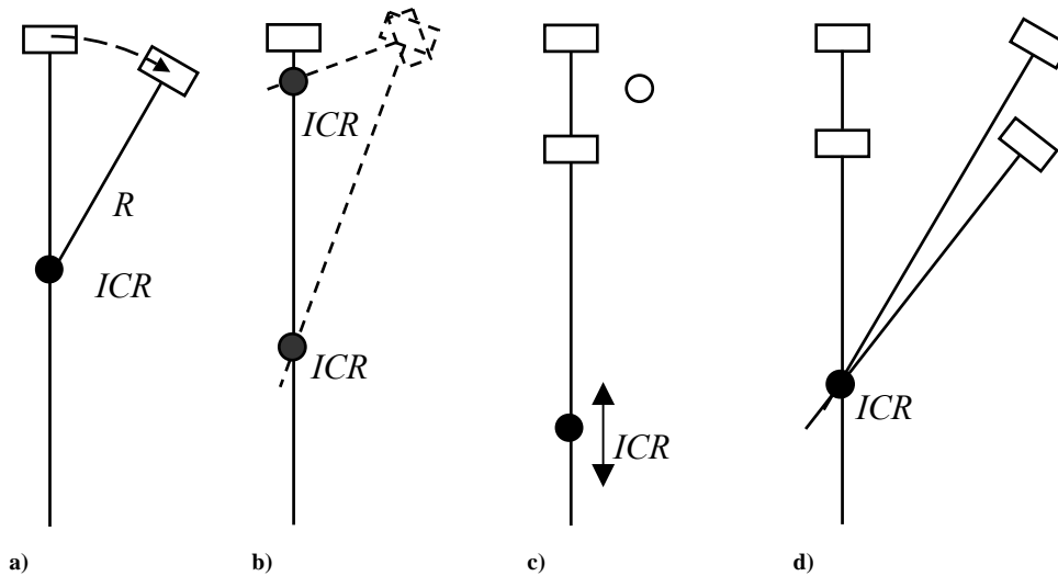
Fig.5.3 Instantaneous Centre of Rotation for: a) Single standard wheel, b) Bike type, c) Differential drive, d) Car drive
