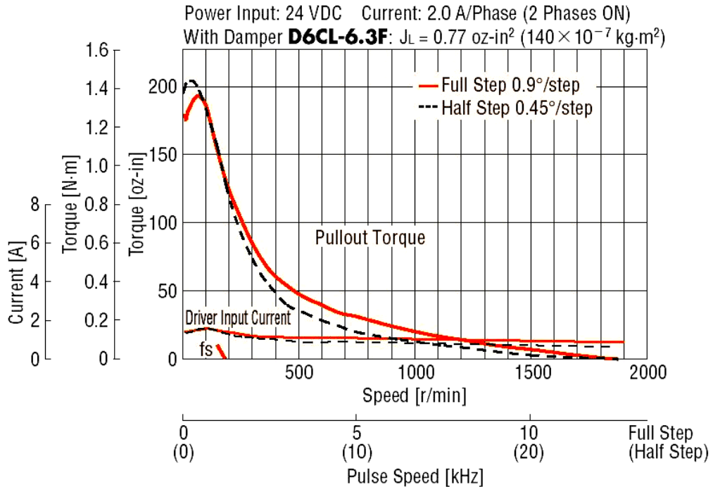
Fig.4.16 Characteristics stepper motor [21]
