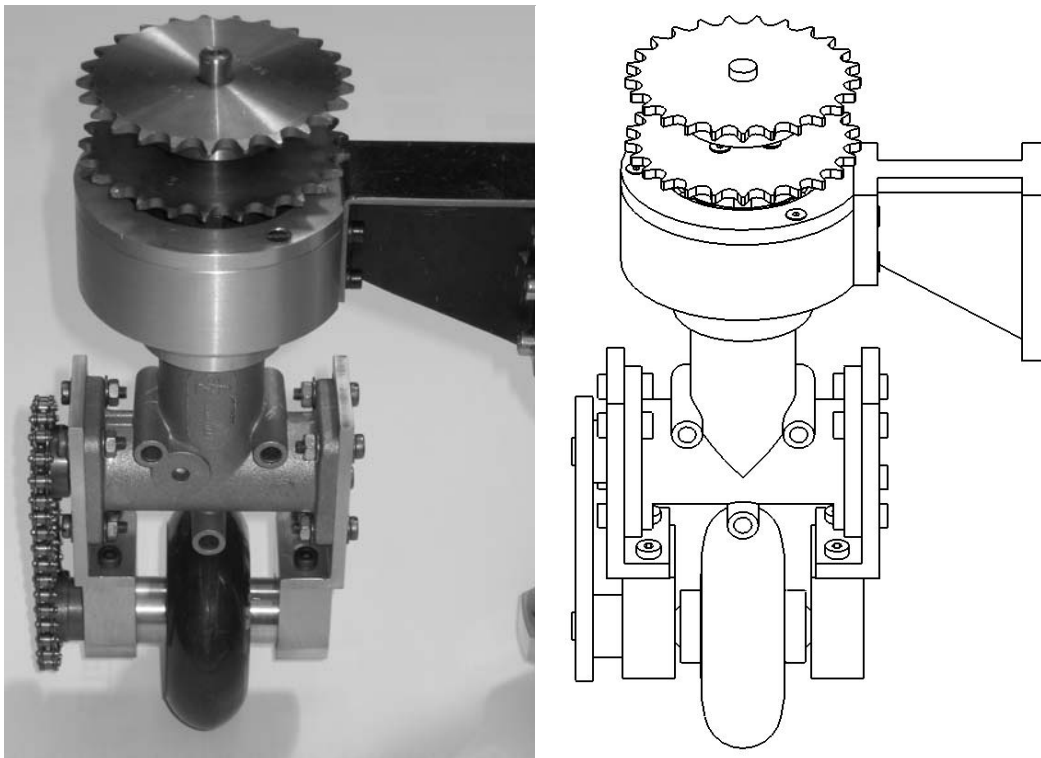
Fig.4.9 Robot's leg
